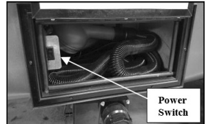
Macerator hose and dump connector
