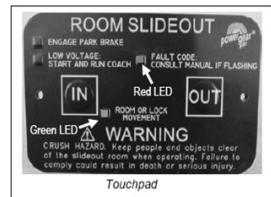
Fig.1 Slideout Controller
