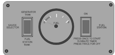
Dual Tank Fuel Gauge & Selector Switch
